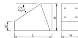
Angled Wedges
